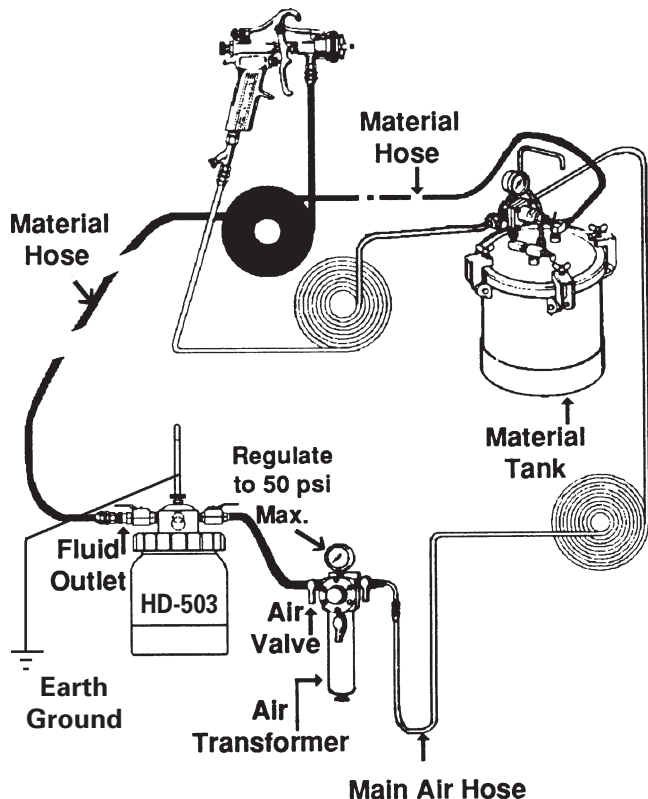
FIGURE 1 - TYPICAL INSTALLATION
